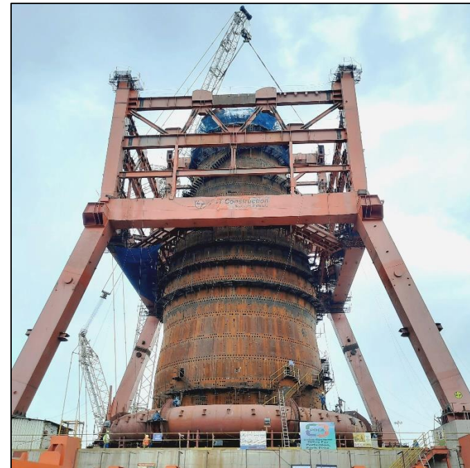
5mtpa expansion: Blast Furnace under construction
