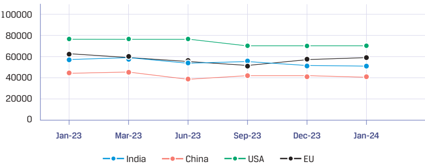
Trends in Global Rebar Prices (₹/T)
